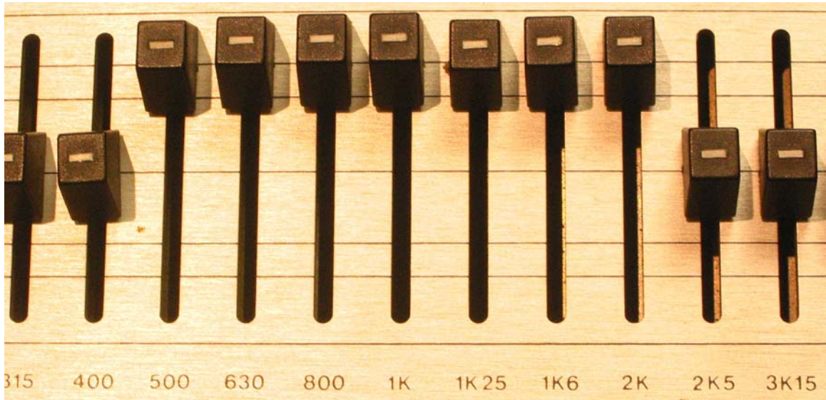
Figure 1: 6 dB boosts from 500 Hz to 2 kHz on analog graphic equalizer
