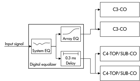
C3 wiring with C4-TOP and C4-SUB
